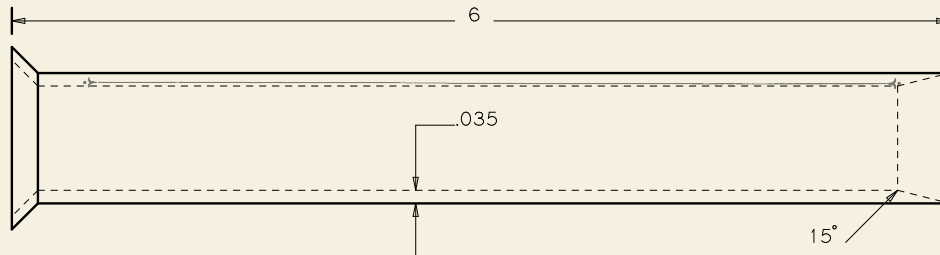
6" long x 0.035 wall flare on inlet end and 15° taper on outlet end
